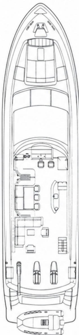
SUN DECK
