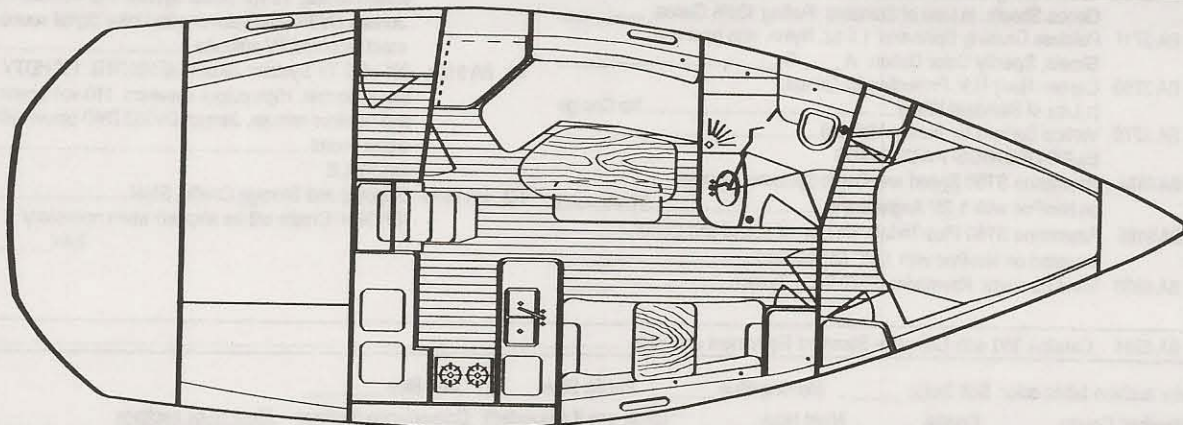
Catalina 350 standard interior layout
