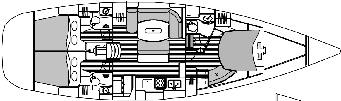
2 AFT CABIN, 1 CENTRAL FORWARD BERTH VERSION CHART TABLE ON STARBOARD
